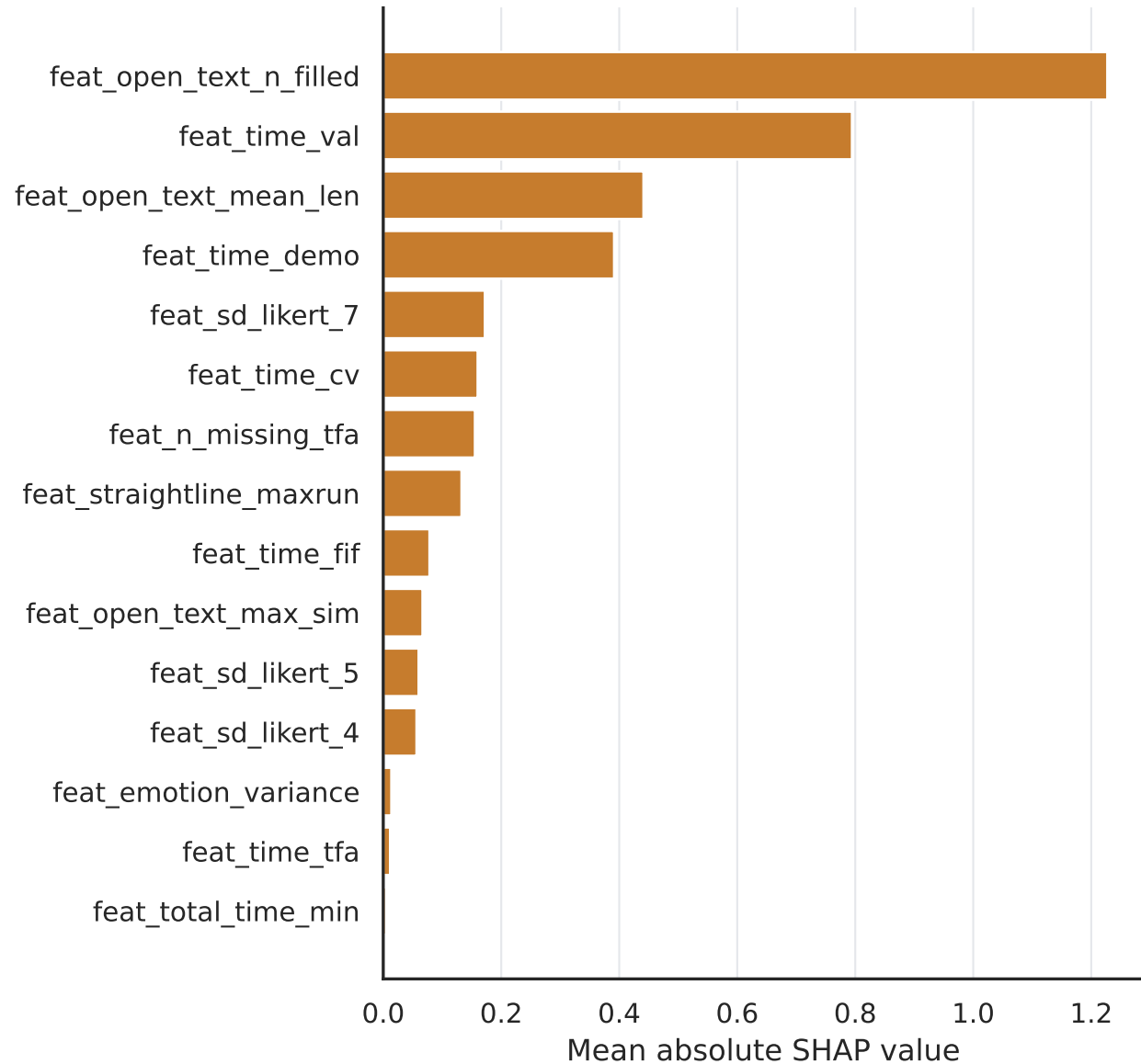
SHAP summary
