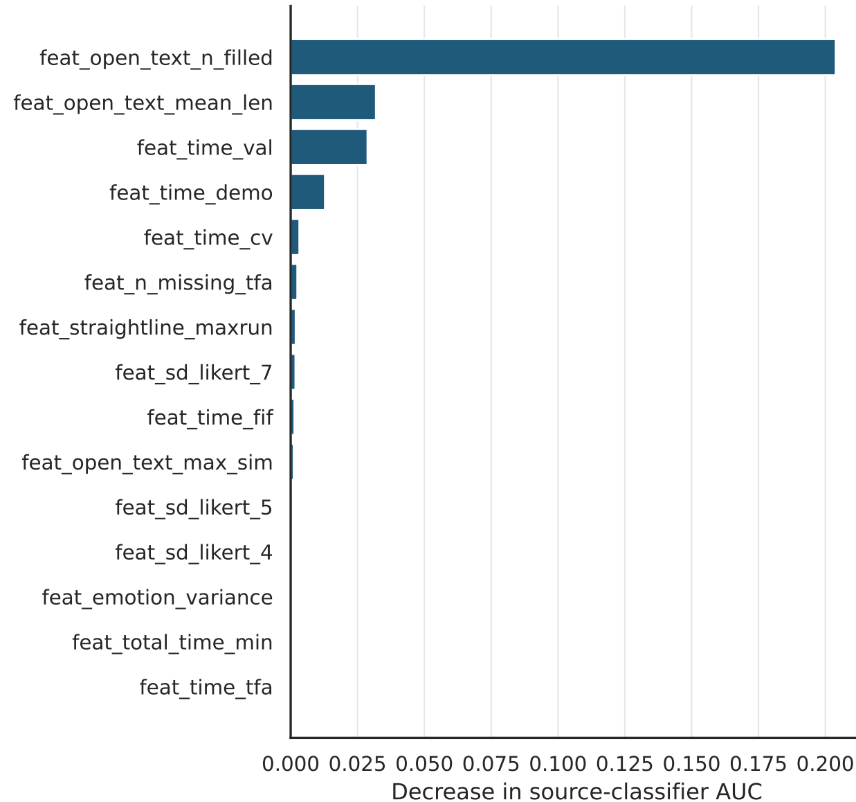
Permutation importance
